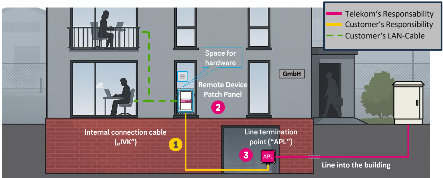
Image 1: Connection between line termination point (“APL”) and remote device (RD).
